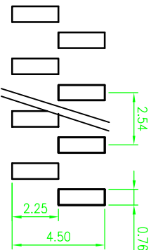
PCB Layout
